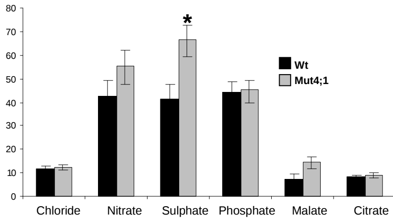
(b) Anion amount ( \mu\text{mol} \cdot 100\text{-seeds}^{-1} )
