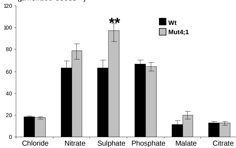
(b) Anion amount ( \mu\text{mol} \cdot 100\text{-seeds}^{-1} )
