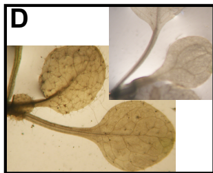
AtHB7 promoter
