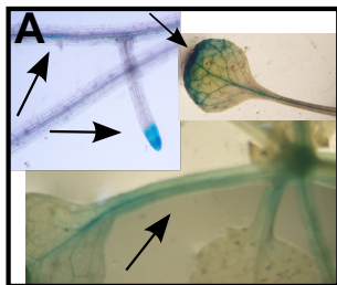
AtHB12 promoter
