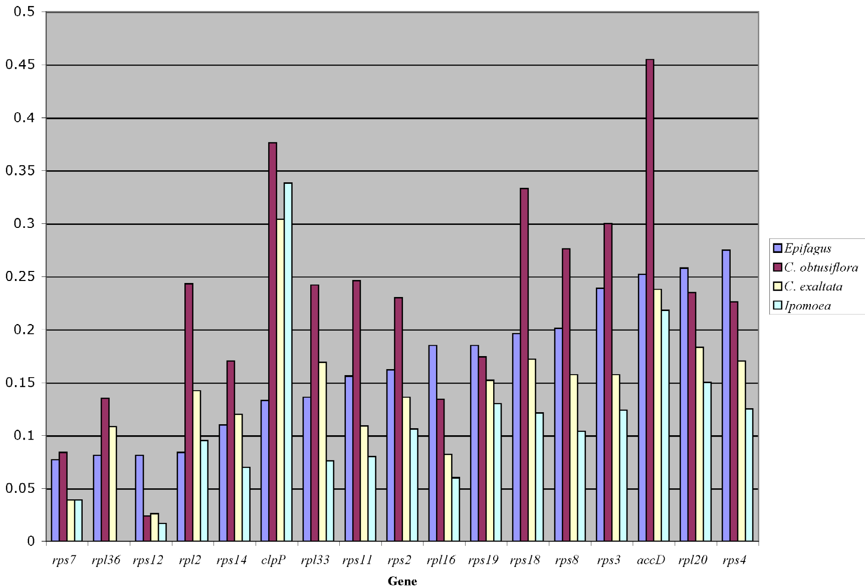
Amino Acid p-distance vs. Panax
