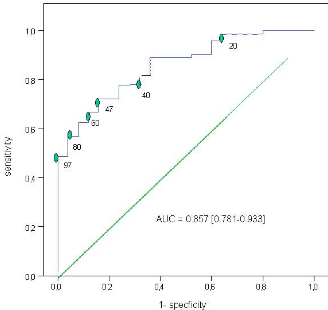
ROC curve
