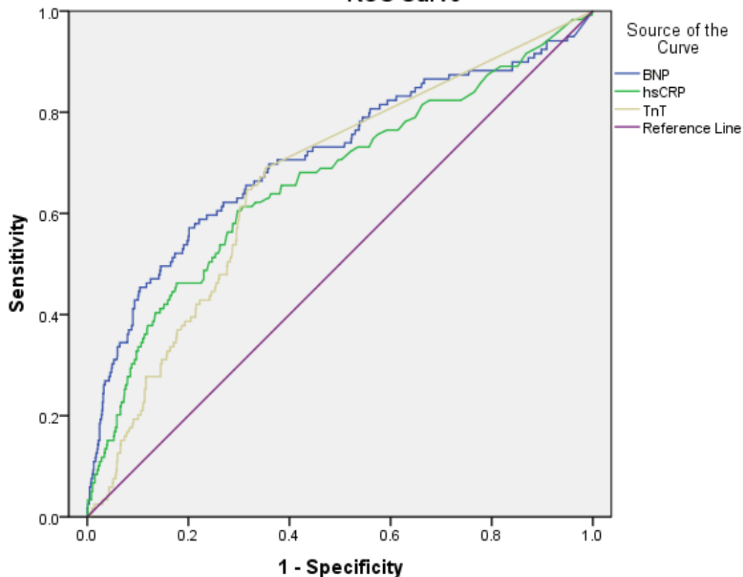
ROC Curve
