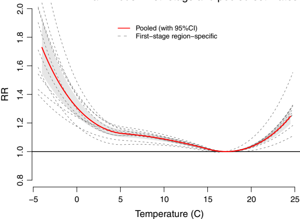
Main model: first-stage and pooled estimates
