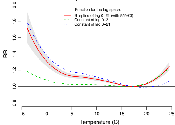
Comparison of alternative models
