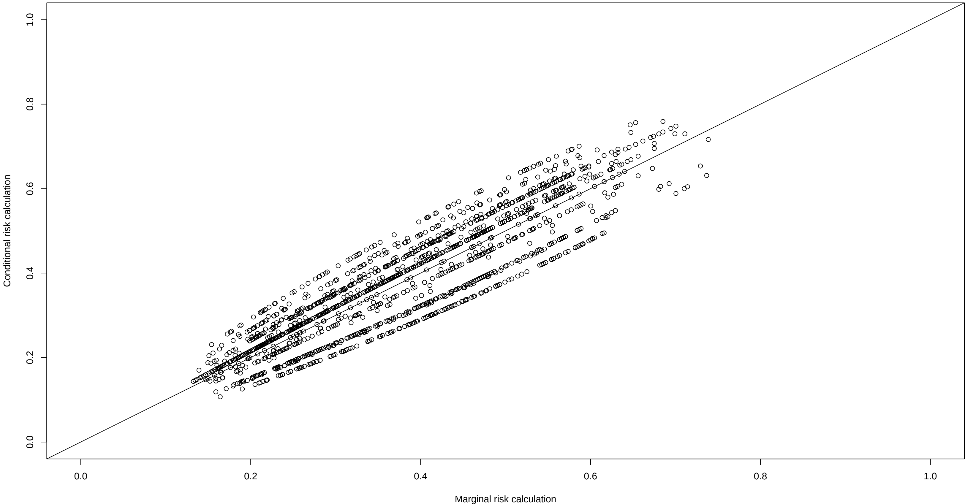
Predicted probabilities
