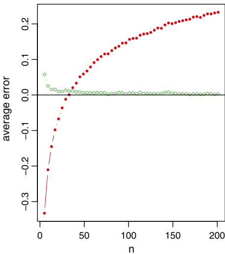
Log-Normal(5,0.5)
