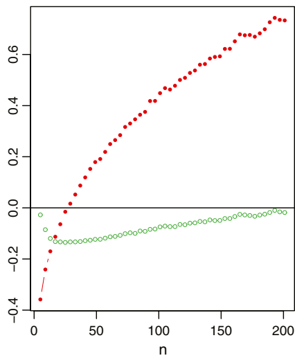
Log-Normal(5,1)
