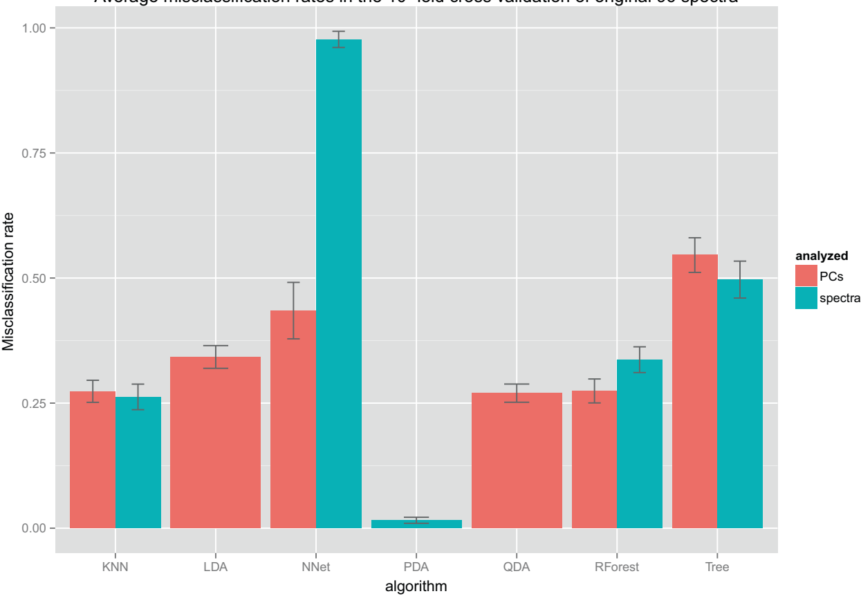
Average misclassification rates in the 10-fold cross validation of original 96 spectra
