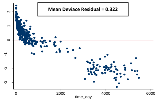
Weibull Model
