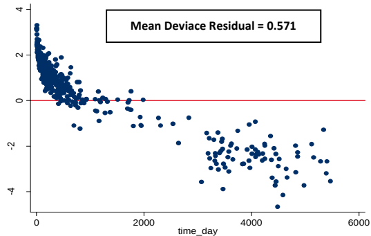
Exponential Model
