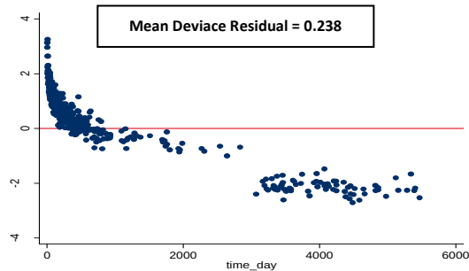
Log-Normal Model
