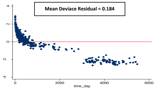
Log-logistic Model
