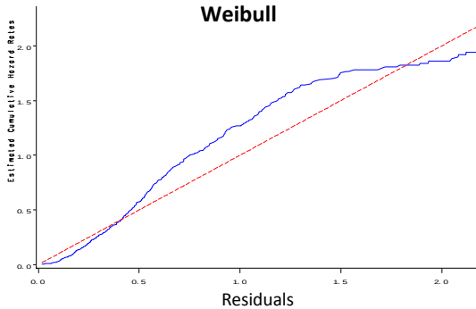
Weibull
