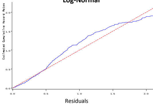
Log-Normal
