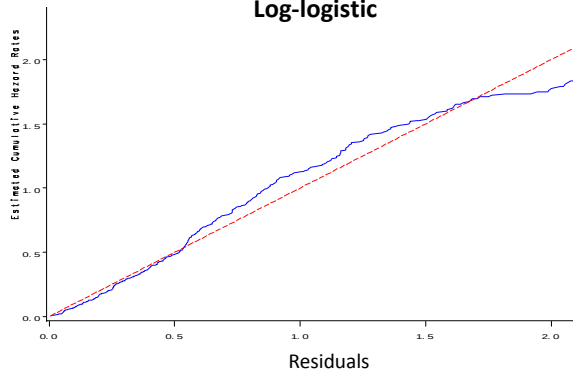
Log-logistic
