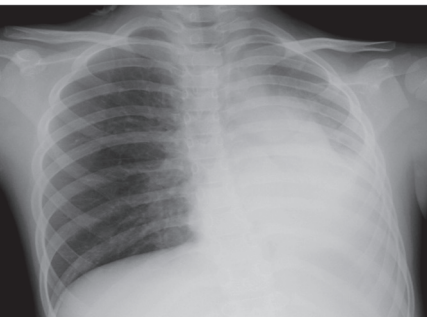
3) Consolidation (32%, n = 64)
