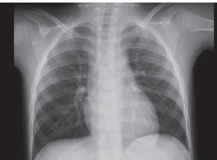
1) normal (23%, n = 46)
