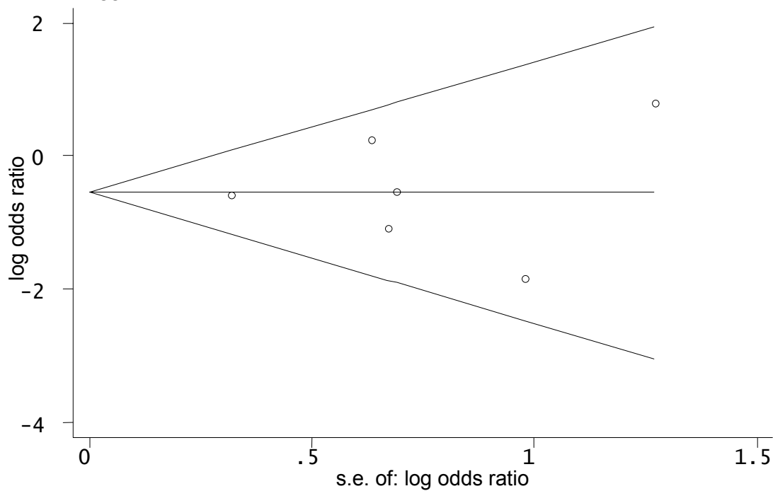
Begg's funnel plot with pseudo 95% confidence limits
