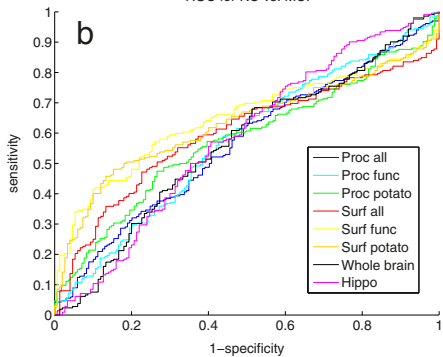
ROC for NC vs. MCI
