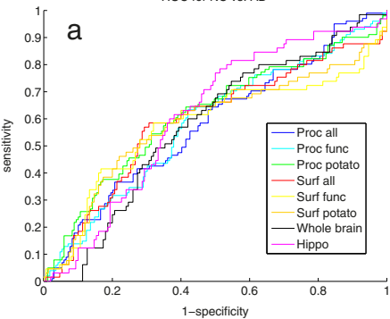
ROC for NC vs. AD
