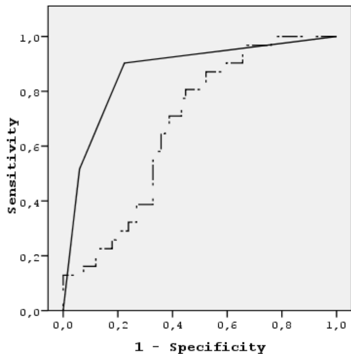
ROC Curve
