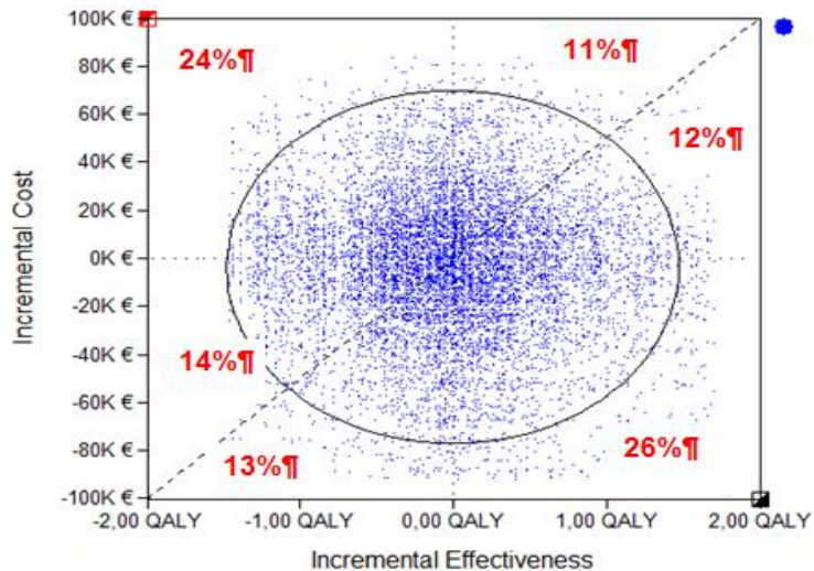
ICE Scatterplot of Arm B vs. Arm A
