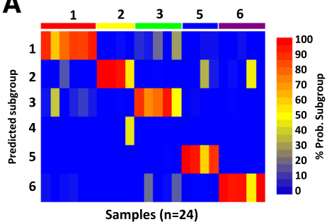
A PAM classifier assigned subgroup
