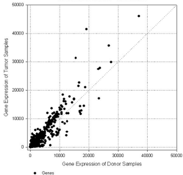
Scatter Plot Tumor vs. Donor / MAS5.0 Data
