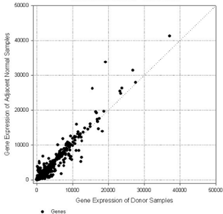
Scatter Plot Adjacent Normal vs. Donor / MAS5.0 Data
