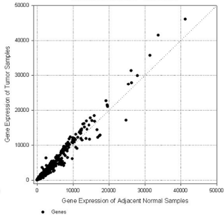
Scatter Plot Tumor vs. Adjacent Normal / MAS5.0 Data
