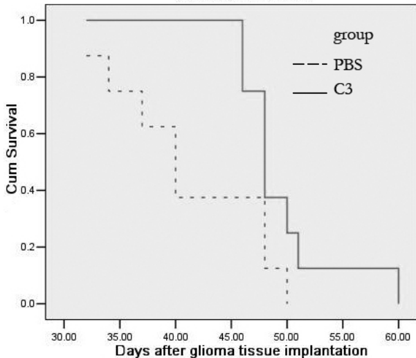
Survival Functions
