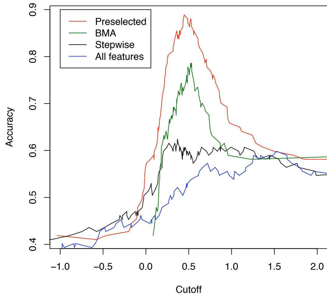
Accuracy Curves, Normal vs. Cancer, Linear Models
