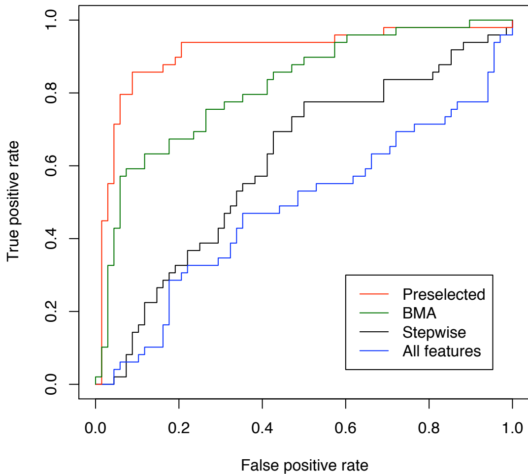
ROC Curve, Normal vs. Cancer, Linear Models
