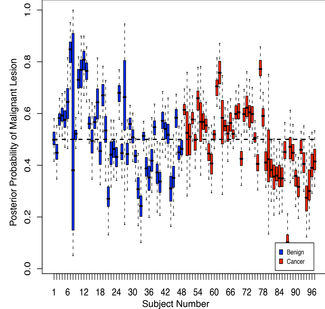
Posterior Predictions for BMA of Probit Models Benign vs. Cancer, Cross-Validation
