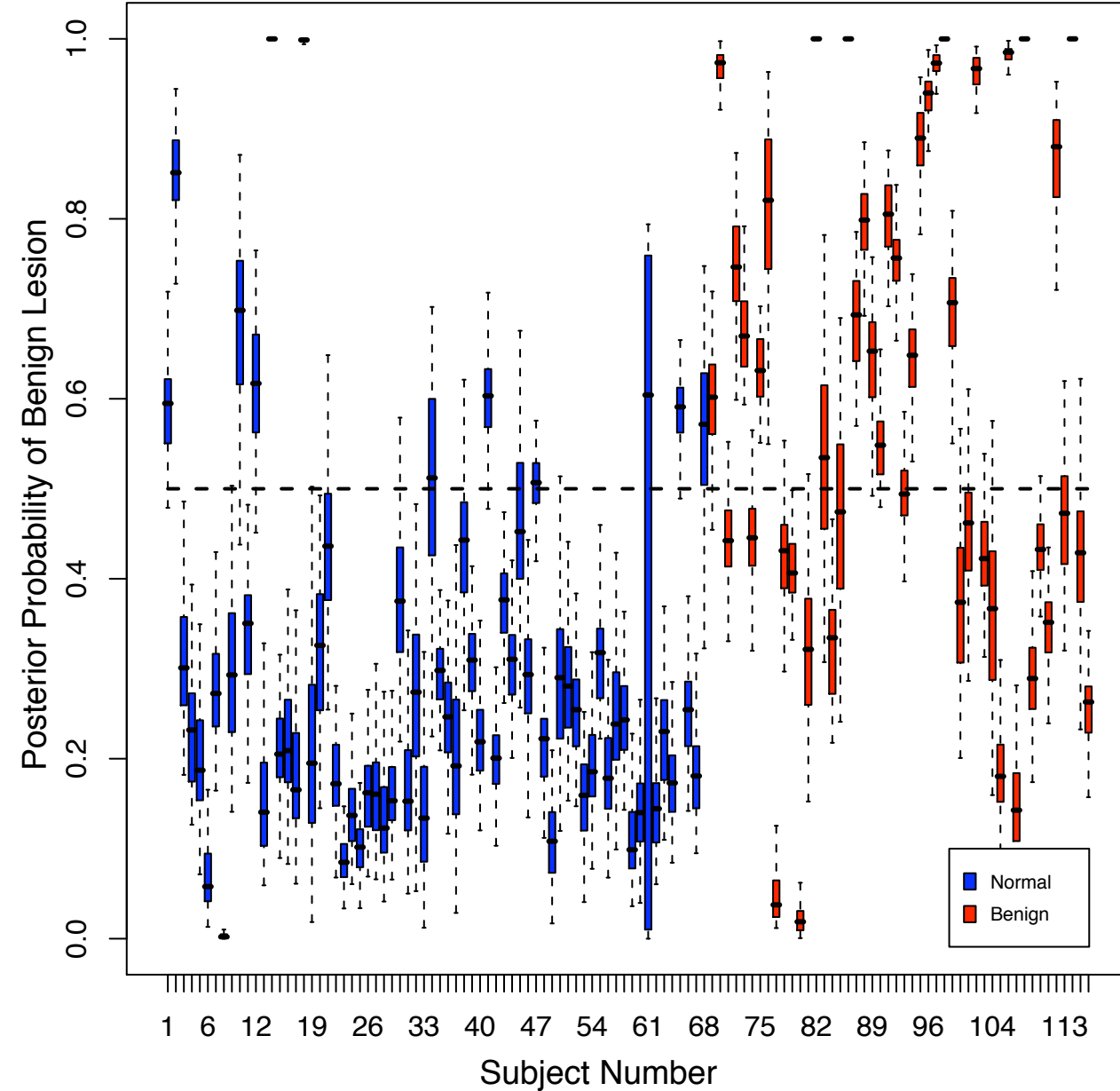
Posterior Predictions for BMA of Probit Models Normal vs. Benign, Cross-Validation
