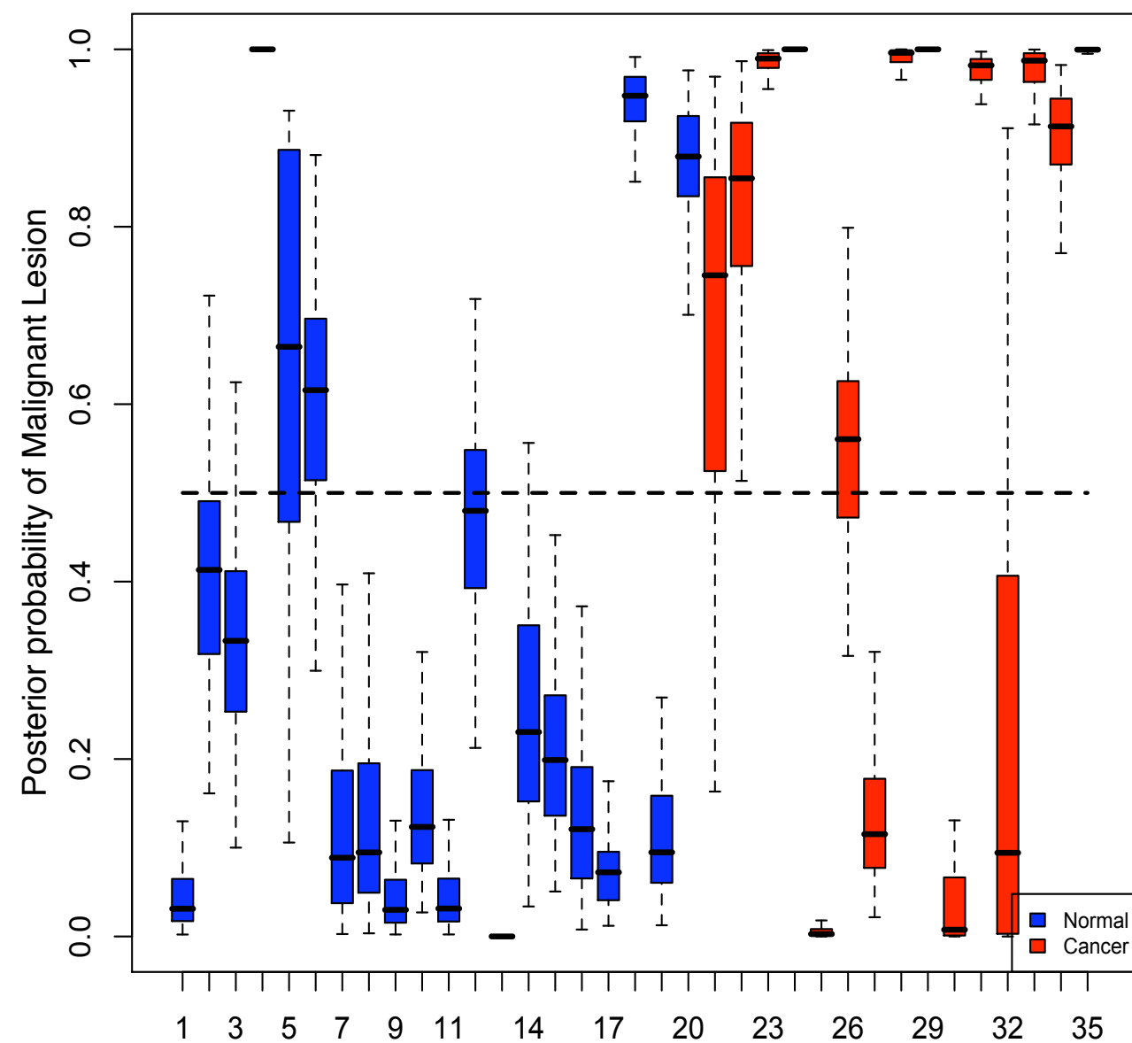
Posterior Predictions for BMA of Probit Models Normal vs. Cancer, Test Set
