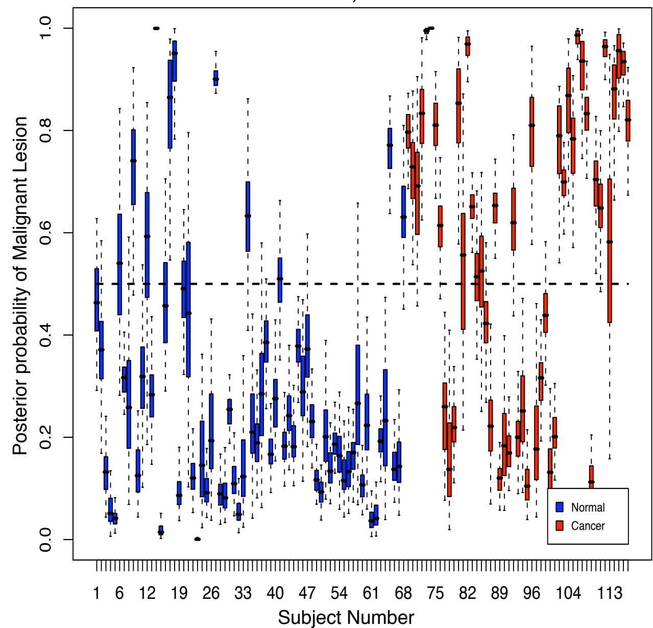
Posterior Predictions for BMA of Probit Models Normal vs. Cancer, Cross-Validation
