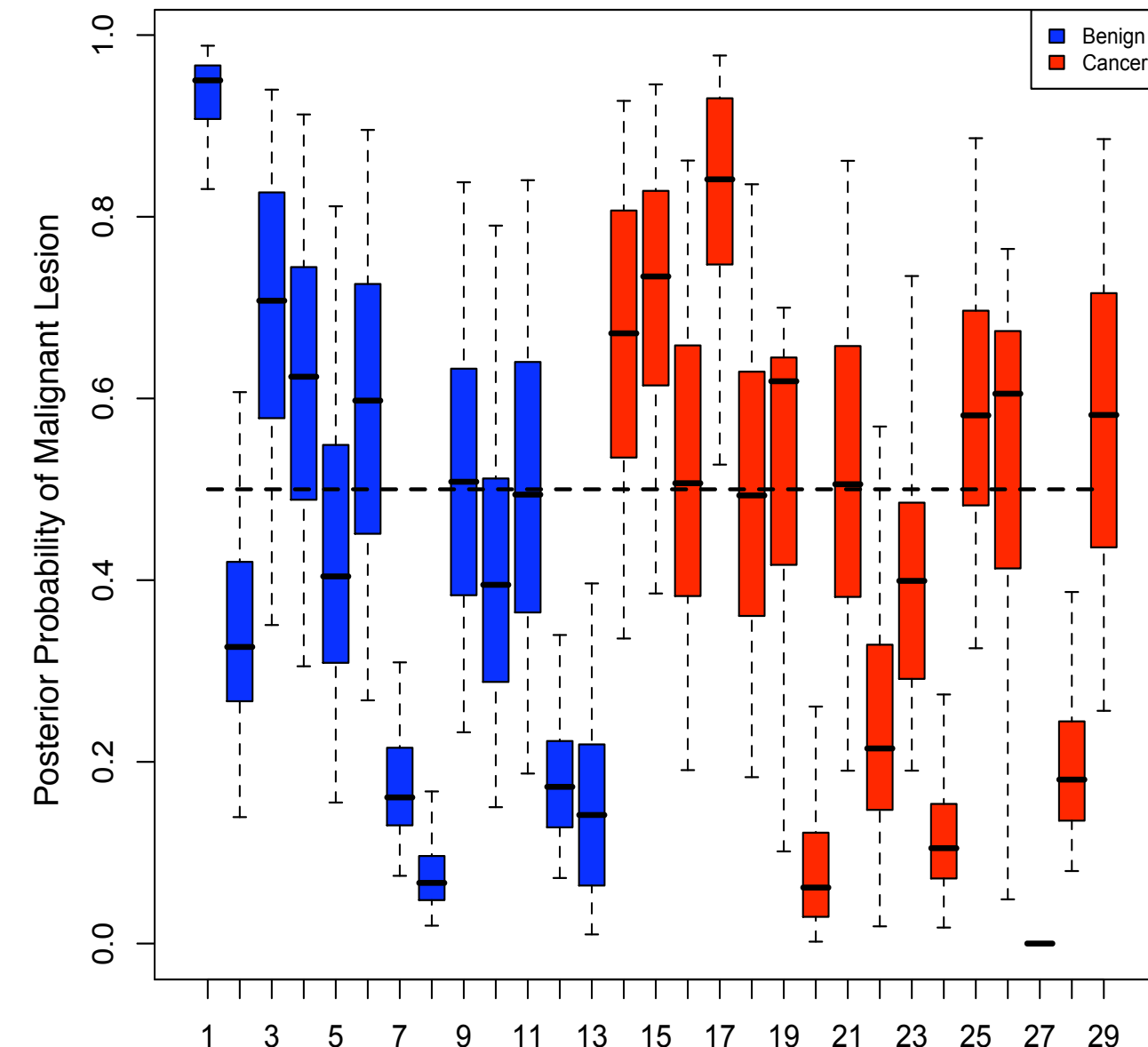
Posterior Predictions for BMA of Probit Models Benign vs. Cancer, Test Set
