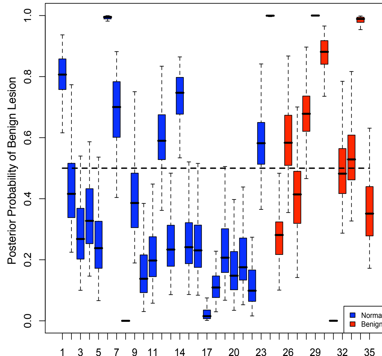
Posterior Predictions for BMA of Probit Models Normal vs. Benign, Test Set
