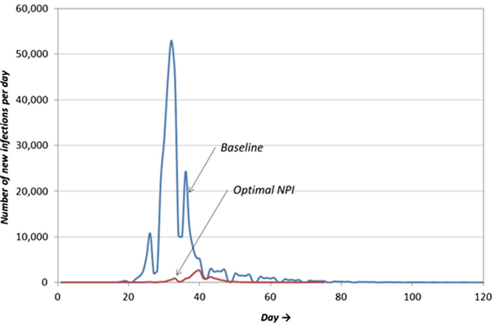
Number of new infections per day for baseline (no intervention) vs. optimal NPI strategy obtained from the 2-level experiment for the low transmissibility scenario
