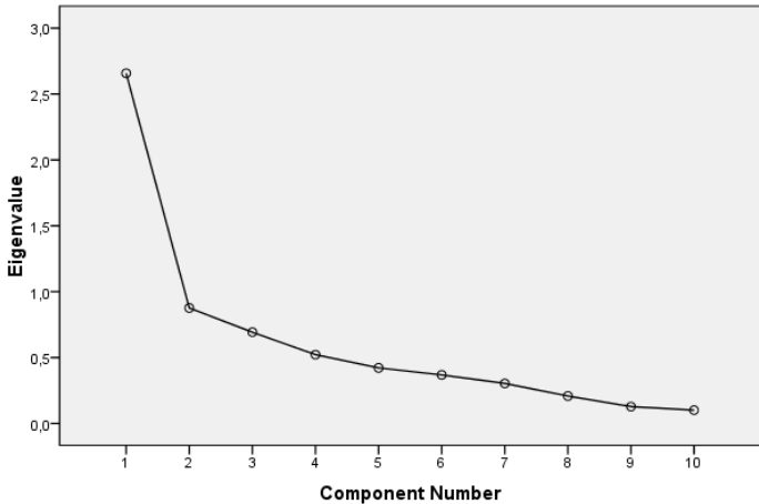
Scree Plot
