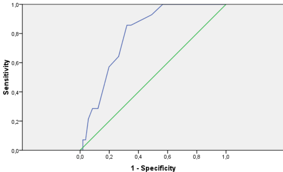
ROC Curve
