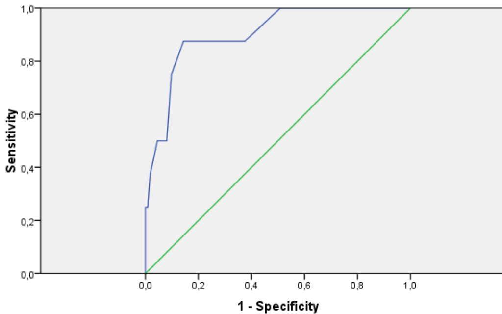
ROC Curve
