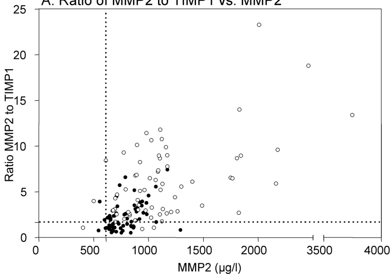
A: Ratio of MMP2 to TIMP1 vs. MMP2
