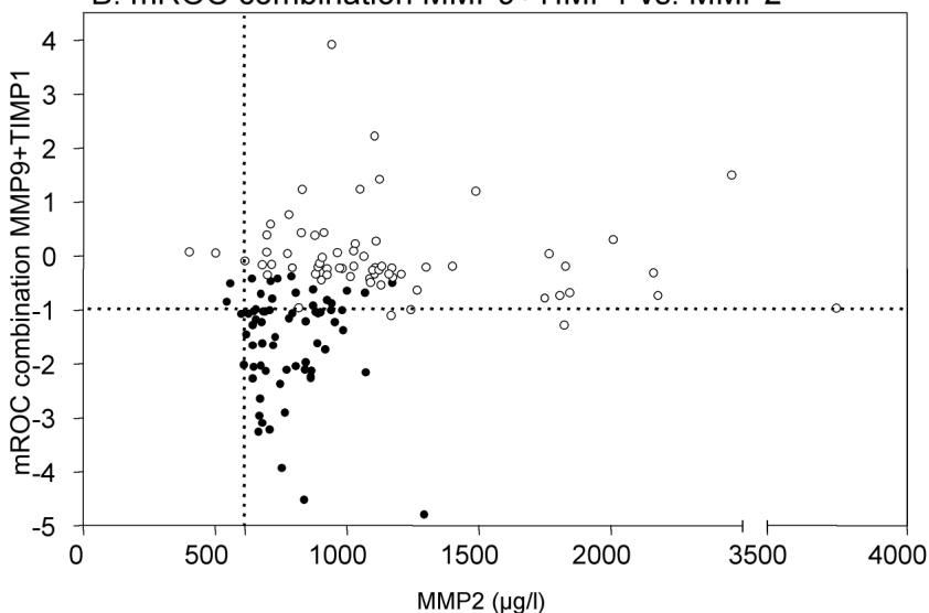
B: mROC combination MMP9+TIMP1 vs. MMP2
