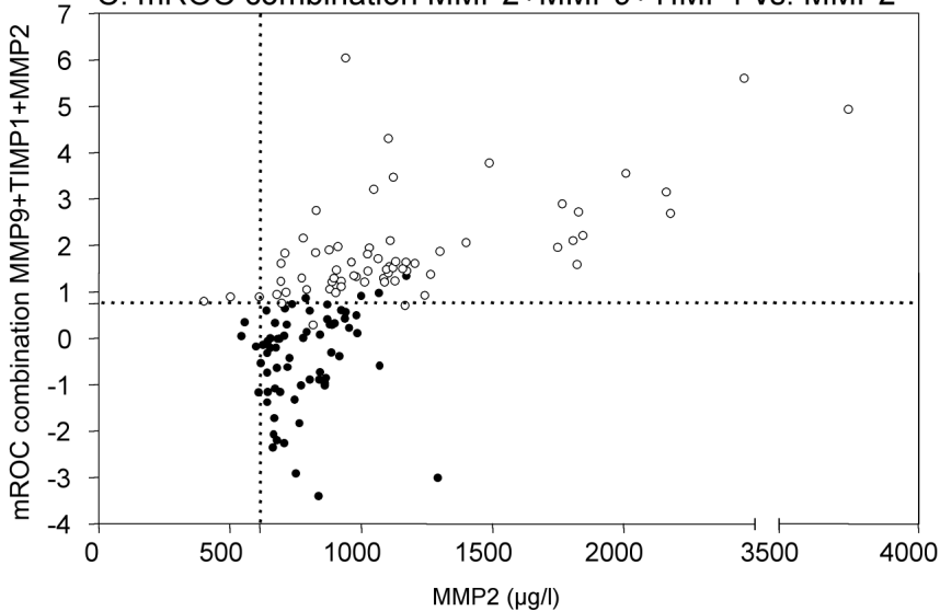
C: mROC combination MMP2+MMP9+TIMP1 vs. MMP2
