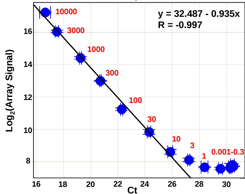
miR-494, Placenta
