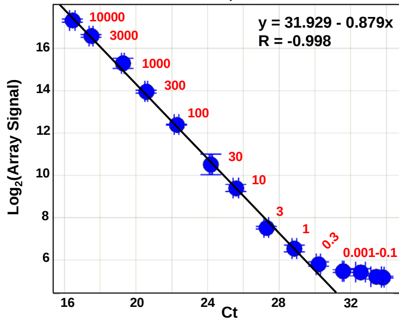
miR-494, Liver
