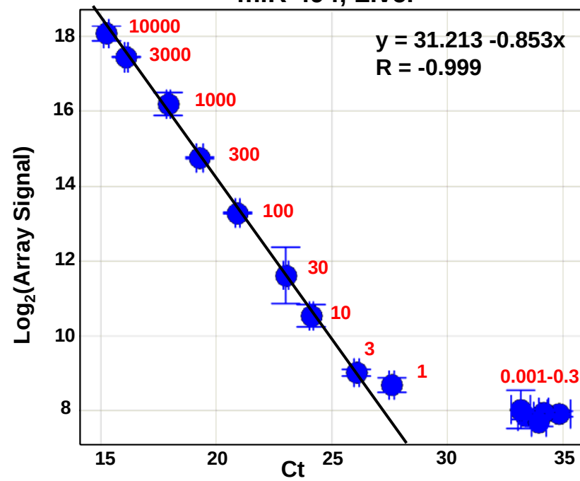
miR-494, Liver
