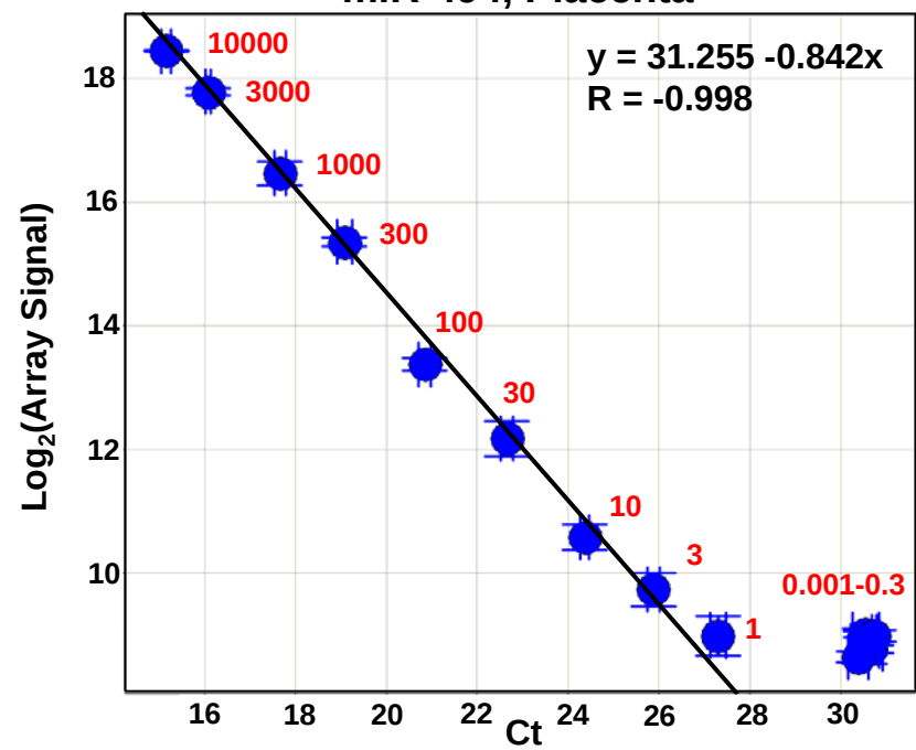
miR-494, Placenta
