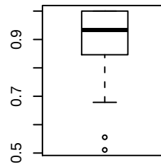
canopy cover
