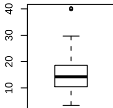
leaves
