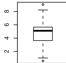
box-cox(gravel)
