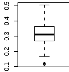
box-cox(LEAF LITTER)
