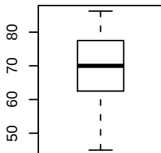
CANOPY COVER
