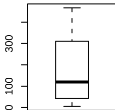
slope
