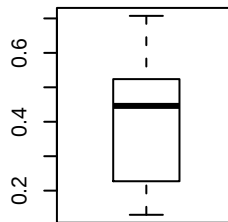
box-cox(width)
