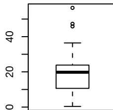
gravel
