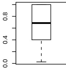
box-cox(canopy cover)
