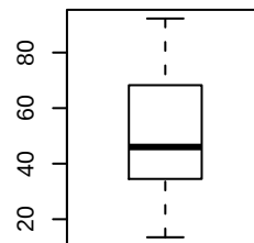
SHRUBS
