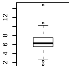
TREES
