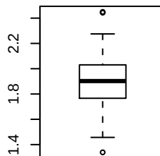
box-cox(leaves)
