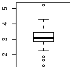
box-cox(TREES)
