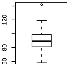
RIPARIAN VEGETATION
