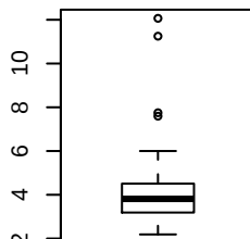
LEAF LITTER
