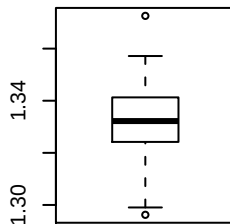
box-cox(RIPARIAN VEG.)
