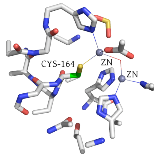
1A7T:A
