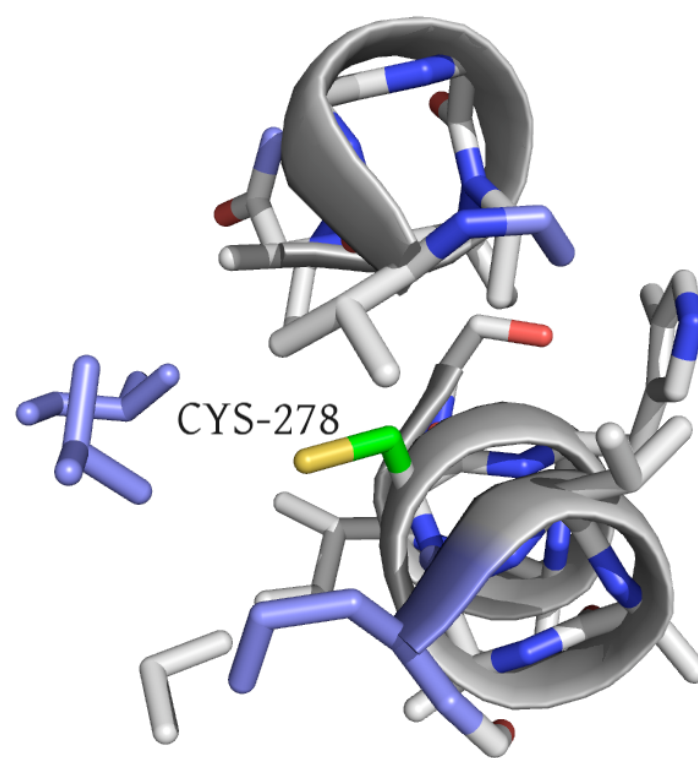
1WA5:B
