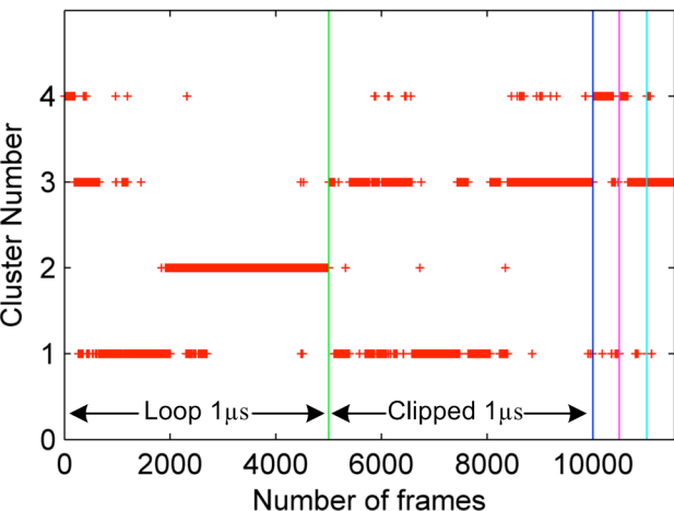
(c) ICL2
