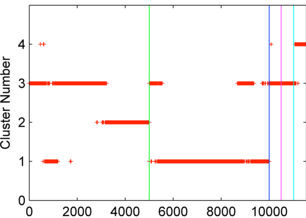
(a) TRANSMEMBRANE
