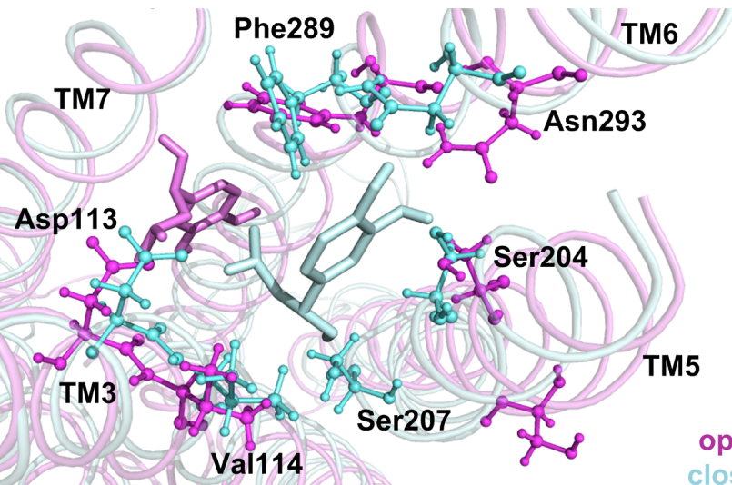
(a) Epinephrine (top view)
