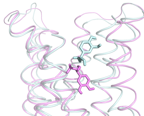
(b) Epinephrine (side view)
