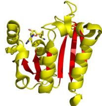
2C7Q_564312
