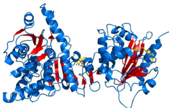
2JHP_fold1a_fold1b
