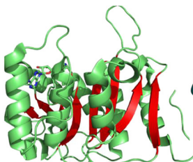
3S1S_7645321
