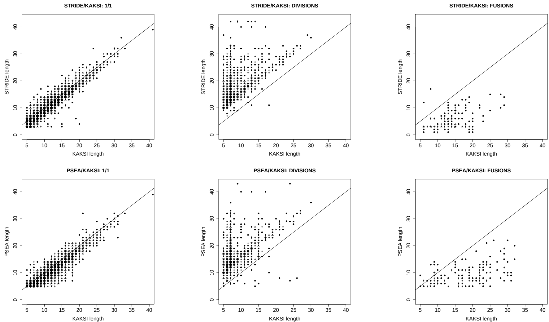
Figure 3: Length for pair of helices when comparing STRIDE and KAKSI assignments, and PSEA and KAKSI assignments. The 3 cases (one-to-one, fusion or division events) are plotted on separate graphs.
