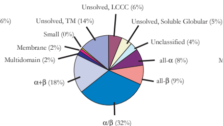
Tropheryma whippelii
