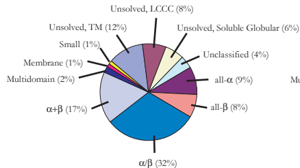
Mycoplasma genitalium
