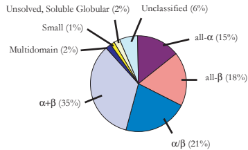
Tropheryma whipplei
