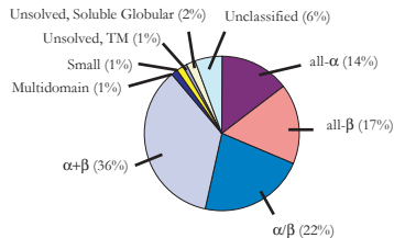
Mycoplasma genitalium
