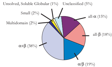
Wigglesworthia glossinidia
