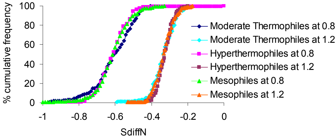
SdiffN computed at different values of vdW tolerance
