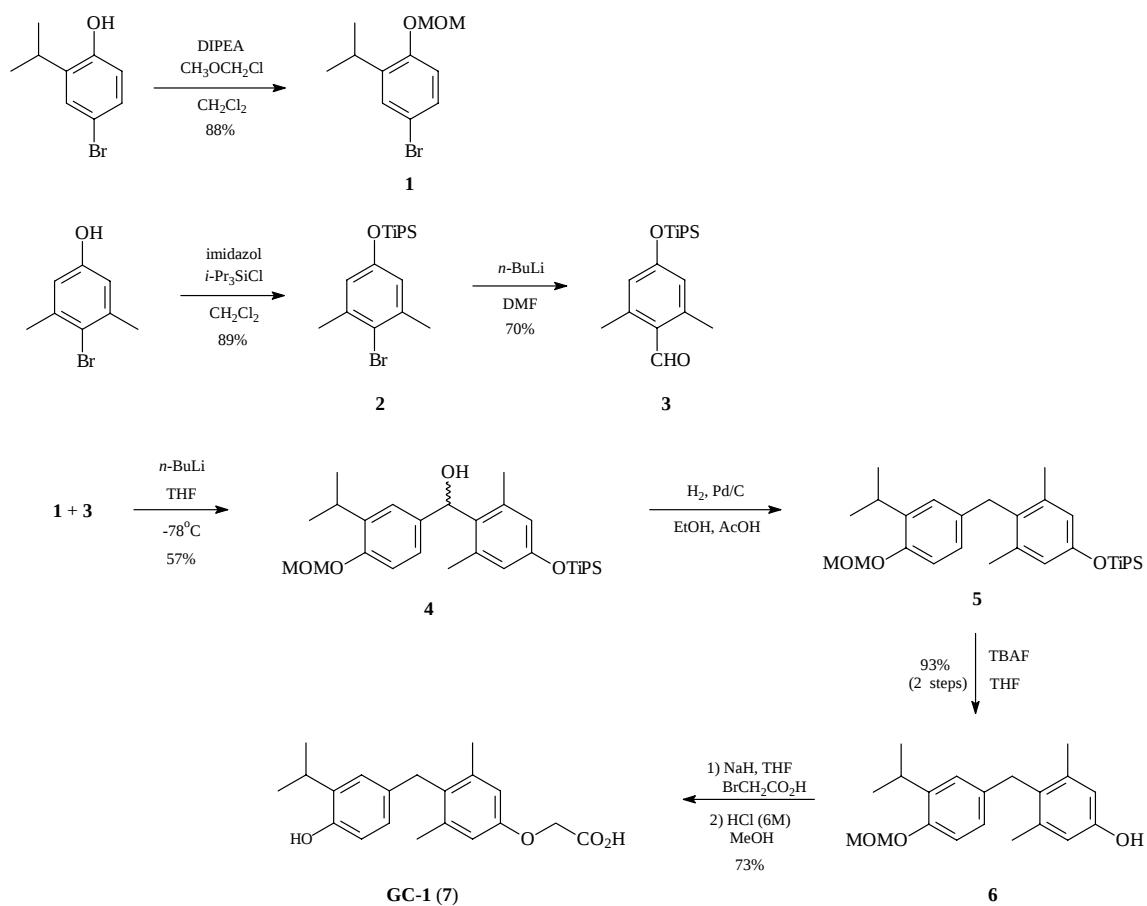
Fig. 2S: Synthetic route of GC-1.
