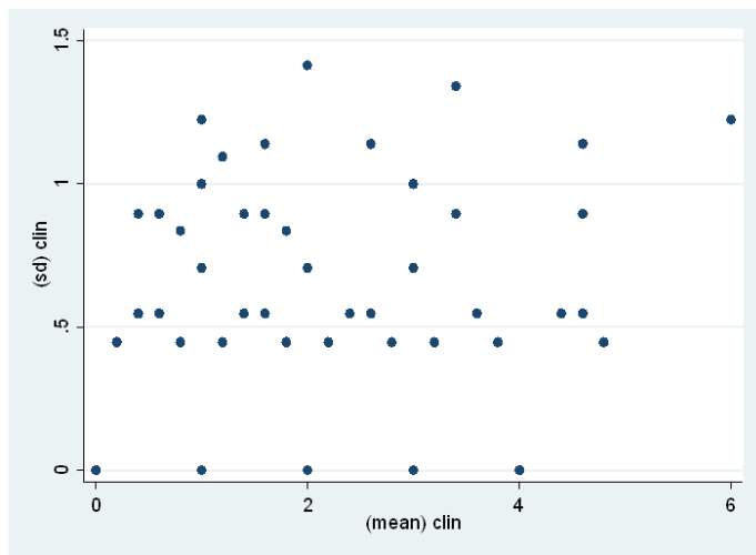
Figure 4b: Scatter Plot of the Standard Deviations against the Means for All Methods in all the 231 10-/11-year-olds
