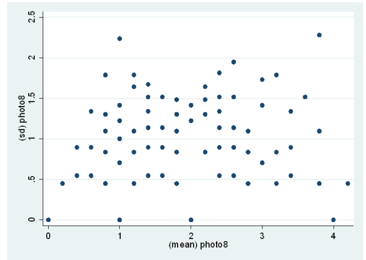
Figure 4b: Scatter Plot of the Standard Deviations against the Means for All Methods in all the 231 10-/11-year-olds
