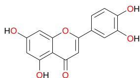
luteolin (19)
