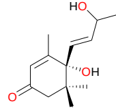
6,9-dihydro-mega-stigmane-3-one (12)
