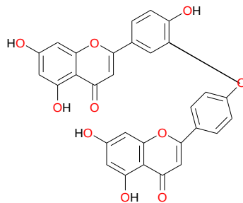
ochnaflavone (17)
