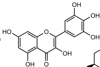
Myricetin
