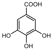
Gallic acid
