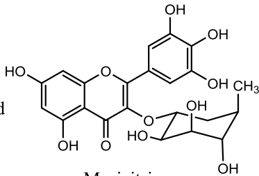
Myricitrin
