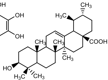
Ursolic Acid
