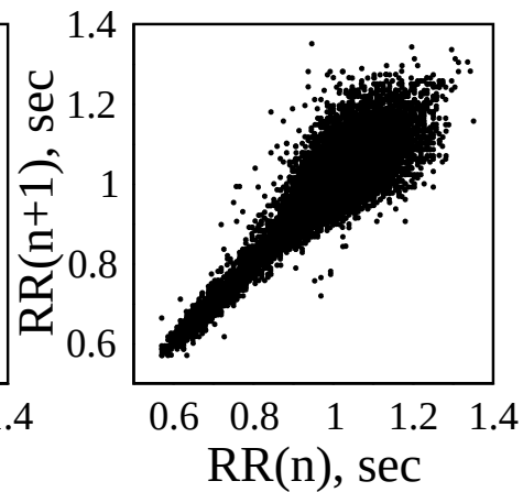
Poincaré plot
