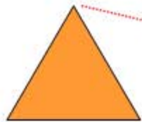
BMC vertex protein
