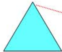
BMC facets protein
