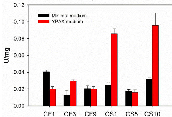
XR, NADPH
