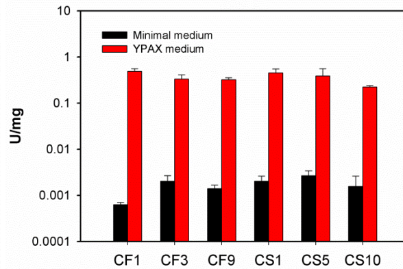
XKS
