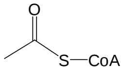
Acetyl-CoA
