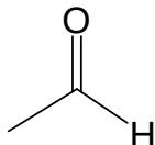
Acetaldehyde
