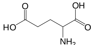
Glutamate
