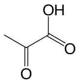
Pyruvate
