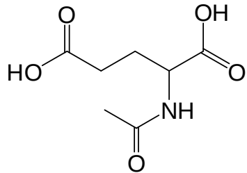
N -Acetylglutamate
