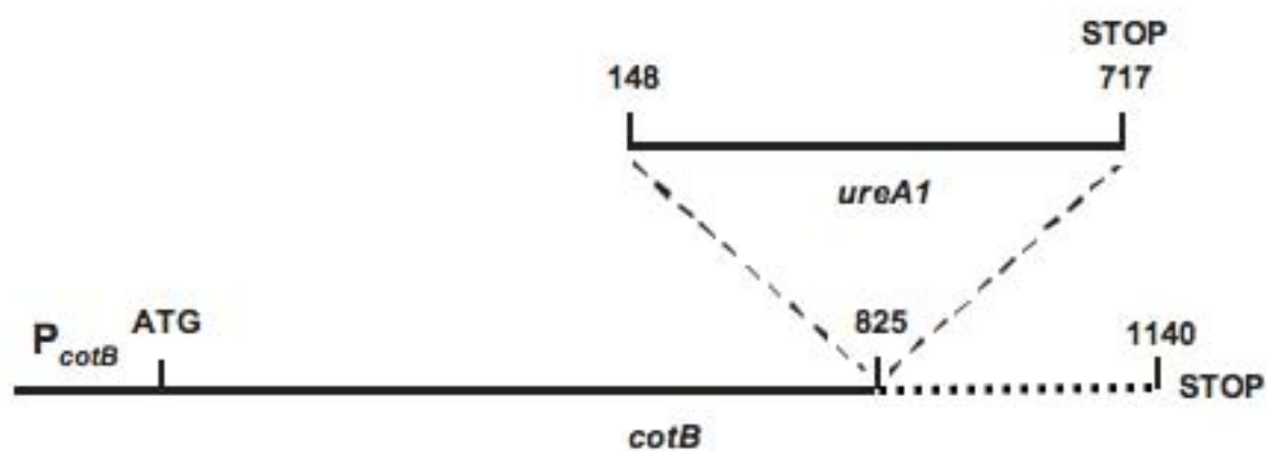
Fusion 1: CotB-UreA1 (52.4 kDa)
