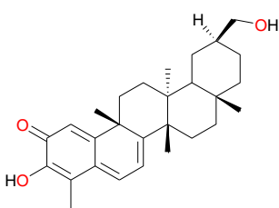
20-Epi-isoiguesterinol ( 101 )
