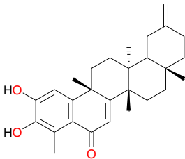
6-Oxoisoiguesterin ( 103 )
