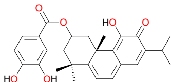
11-Hydroxy-2 \alpha -(3,4-dihydroxybenzoyloxy)abieta -5,7,9(11),13-tetraene-12-one ( 114 )
