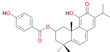
11-Hydroxy-2 \alpha -(4-hydroxybenzoyloxy)-abieta- 5,7,9(11),13-tetraene-12-one ( 113 )
