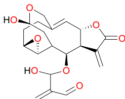
Hydroxyvernolide (124)
