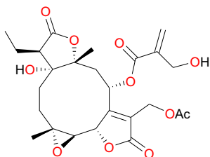
16,17-Dihydrobrachycalyxolide (125)
