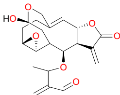
Vernolide (123)
