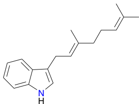
3-Geranylindole (7)
