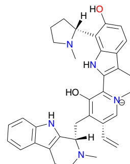
Chrysopentamine (19)
