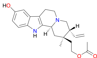
17-O-acetyl,10-hydroxycorynantheol (10)
