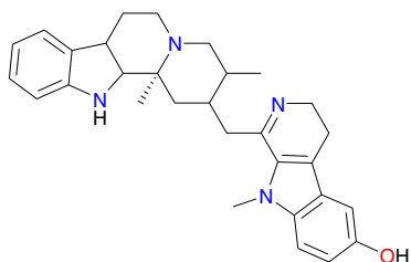
10'-Hydroxyusambarensine (16)
