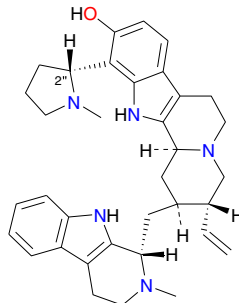
Strychnopentamine (17)
