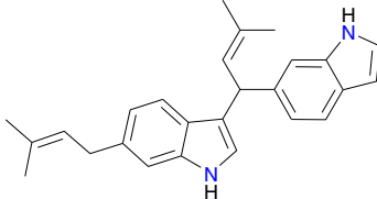
Annonidine F(2)
