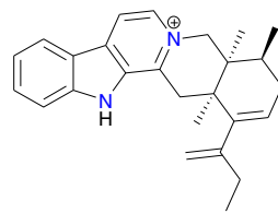
Alstonine (15)
