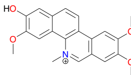
Fagaronine (14)
